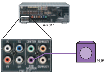
Figure 18 – Subwoofer Connection
