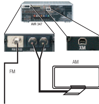
Figure 19 – Antenna Connections
