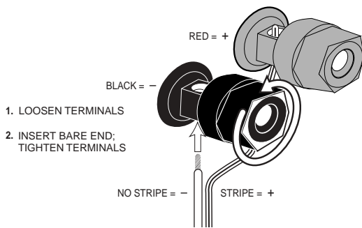
FIGURE 5 – This example shows how to connect bare wires to the terminals. Banana plugs may also be inserted directly into the rear of the connector.
