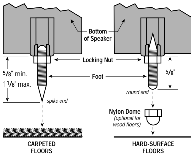
FIGURE 4 – This cross section shows how to install a foot onto the bottom of an Entra floorstanding speaker.
