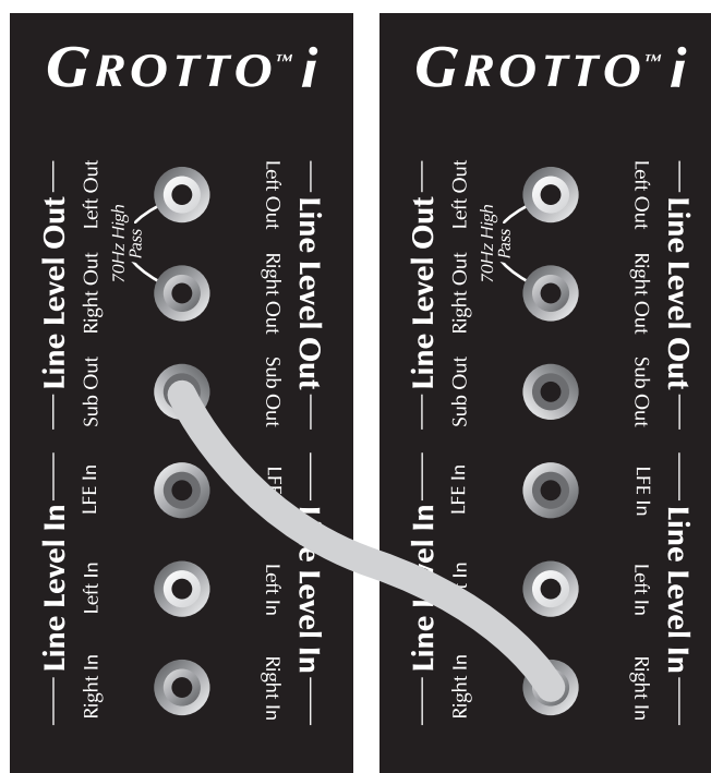
Figure 11. Using multiple Grotto i. Right/Left option.. Primary sub on right. Additional sub on left.
