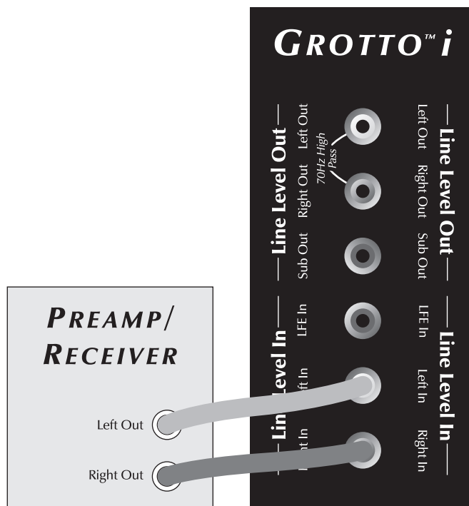
Figure 4. Signal connection for 2-channel mode.
