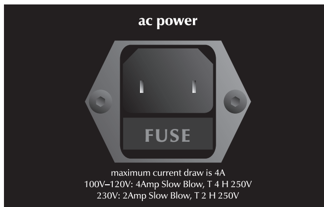
Figure 12. Grotto i's Fuse, and AC Power receptacle.
