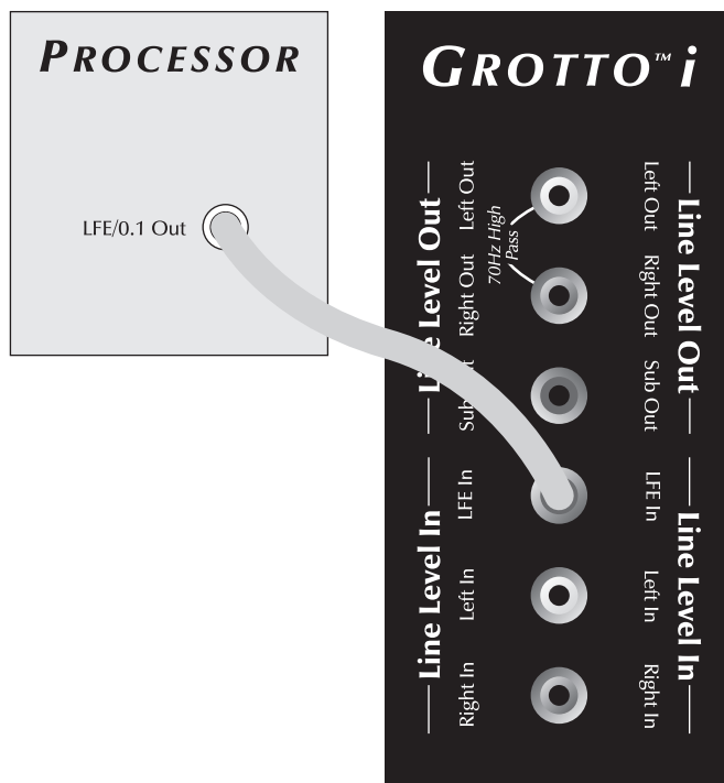
Figure 5. Signal connection for multi-channel mode.
