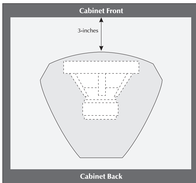
Figure 14. Placing the Grotto i in a cabinet requires a minimum of three inches of open space on the front, left and right.
