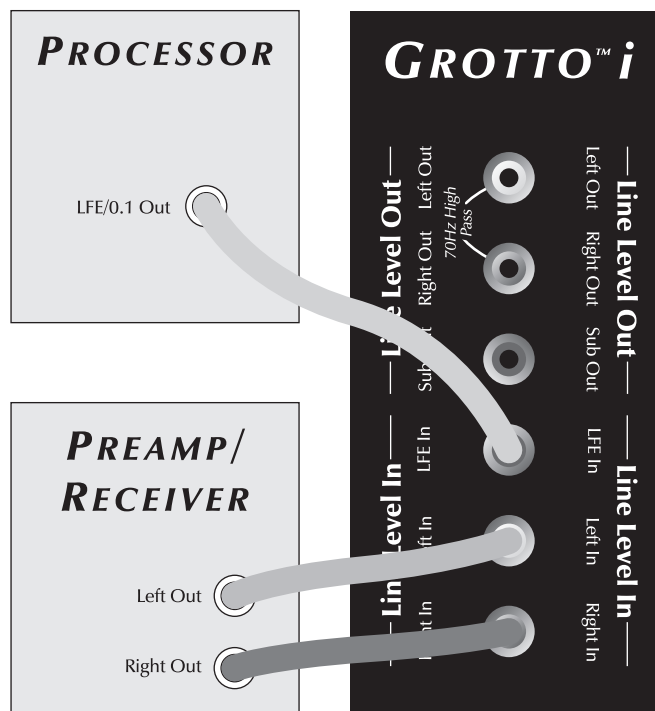
Figure 6. Signal connection for 2-channel/multi-channel mode.
