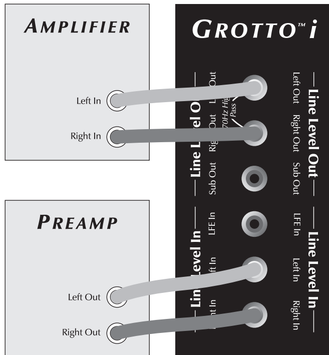
Figure 8. Signal connection for 2-channel mode with 2-channel output.
