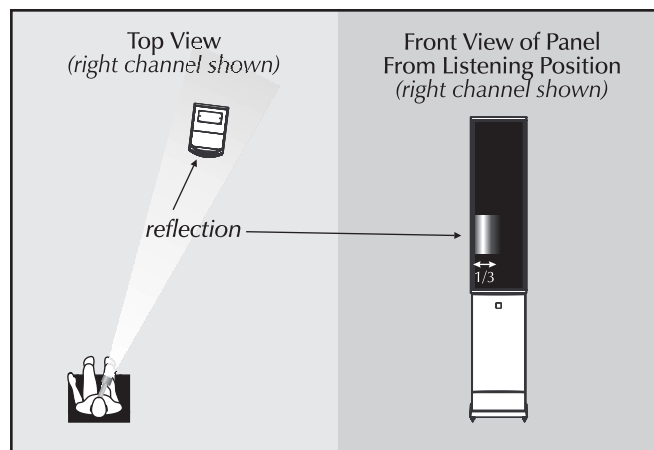
Figure 2. Flashlight toe-in technique.
