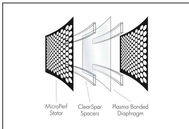
Figure 14. Cut away view of an electrostatic transducer. Notice the simplicity due to minimal parts usage.
