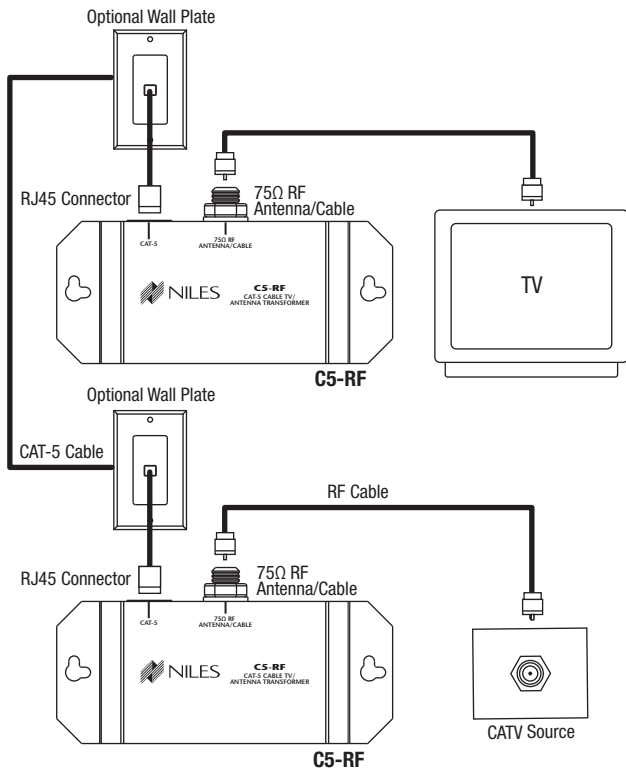
C5-RF Balun Connection Diagram
