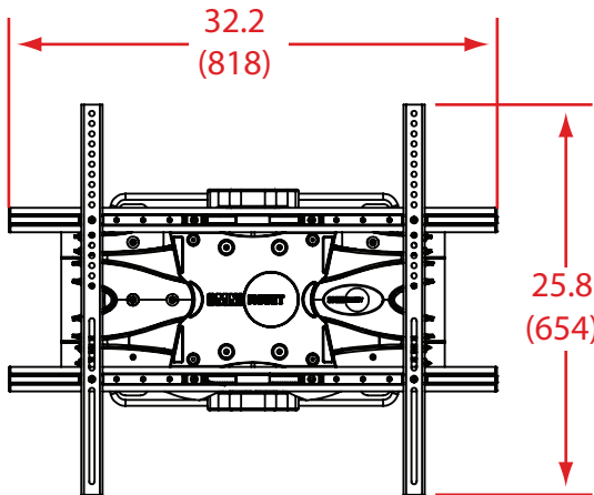
FRONT VIEW WITH ADAPTERS
