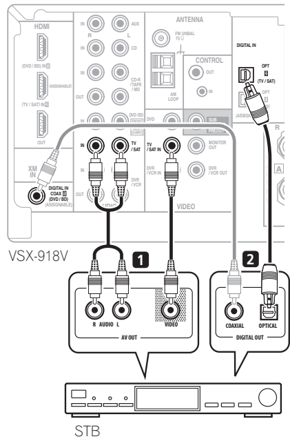
The illustration shows the VSX-918V, but connections for the VSX-818V are the same.
