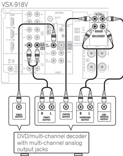
The illustration shows the VSX-918V, but connections for the VSX-818V are the same.
