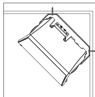
FIGURE 15: Installation of the 45° bracket.
