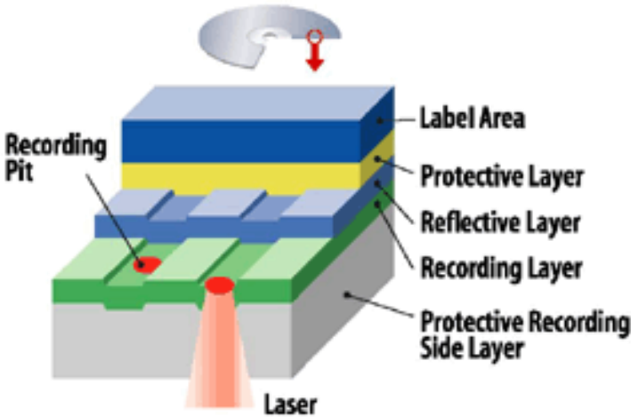
CD-R Structural Cross Section
