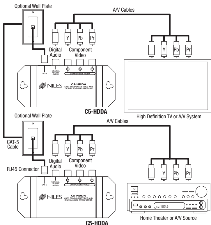
C5-HDDA Balun Connection Diagram
