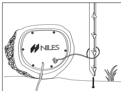
Figure 12 Security Stake Attachment to Cable
