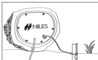
Figure 13 Security Stake Driven into Ground
